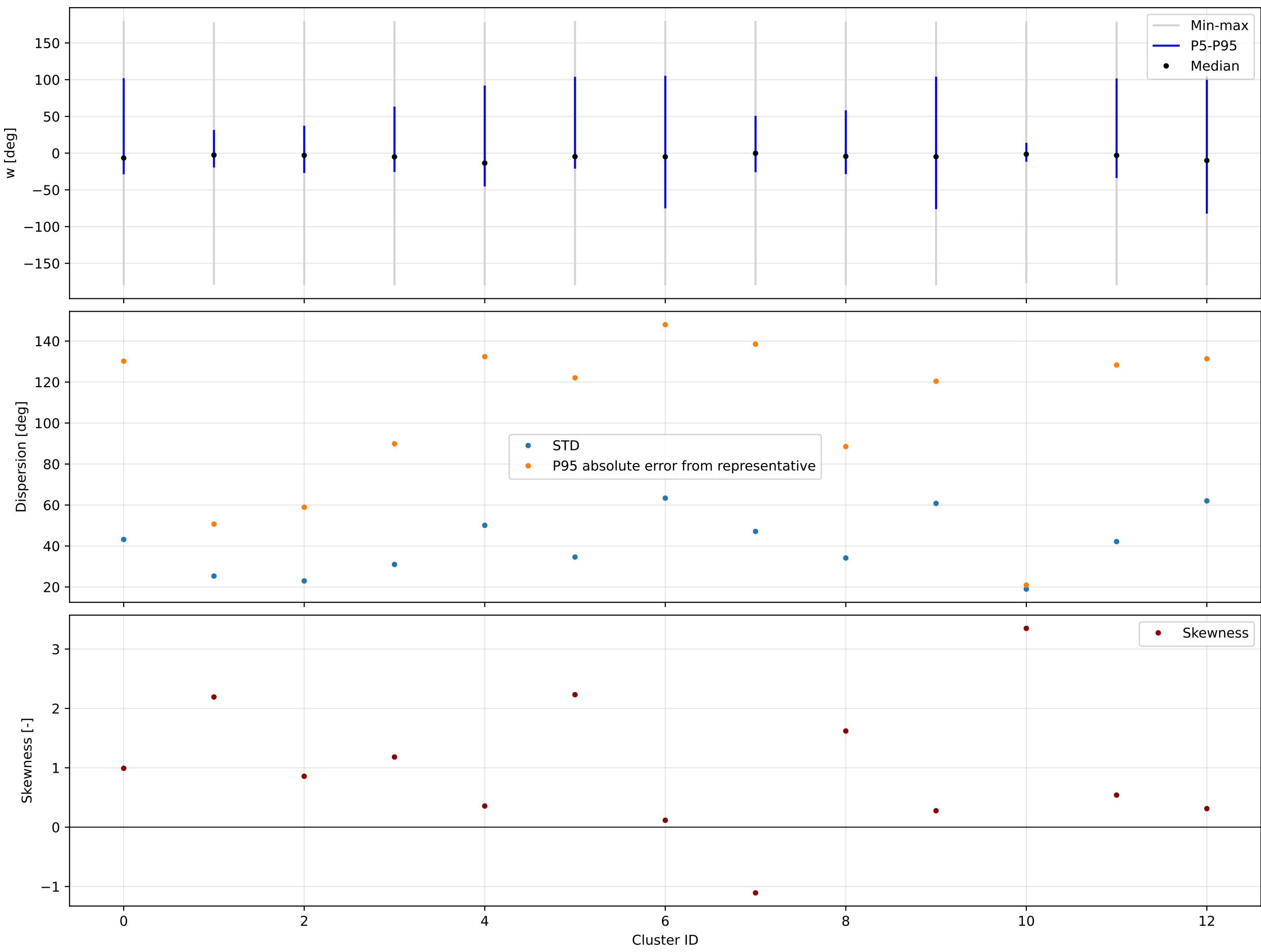
K=13 | forward | w | valid=194058/194124 | offsets from each cluster circular mean
