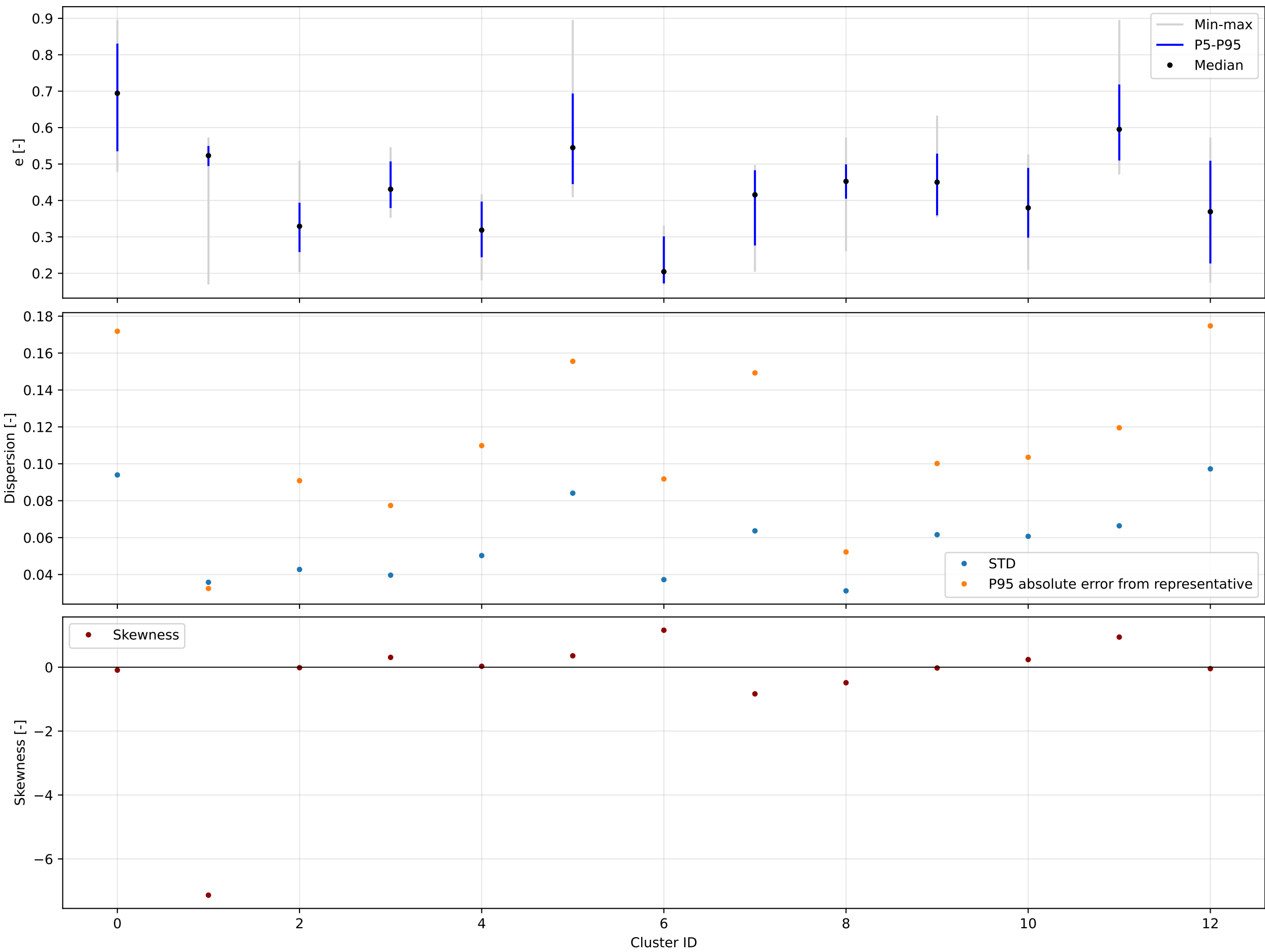
K=13 | backward | e | valid=194124/194124
