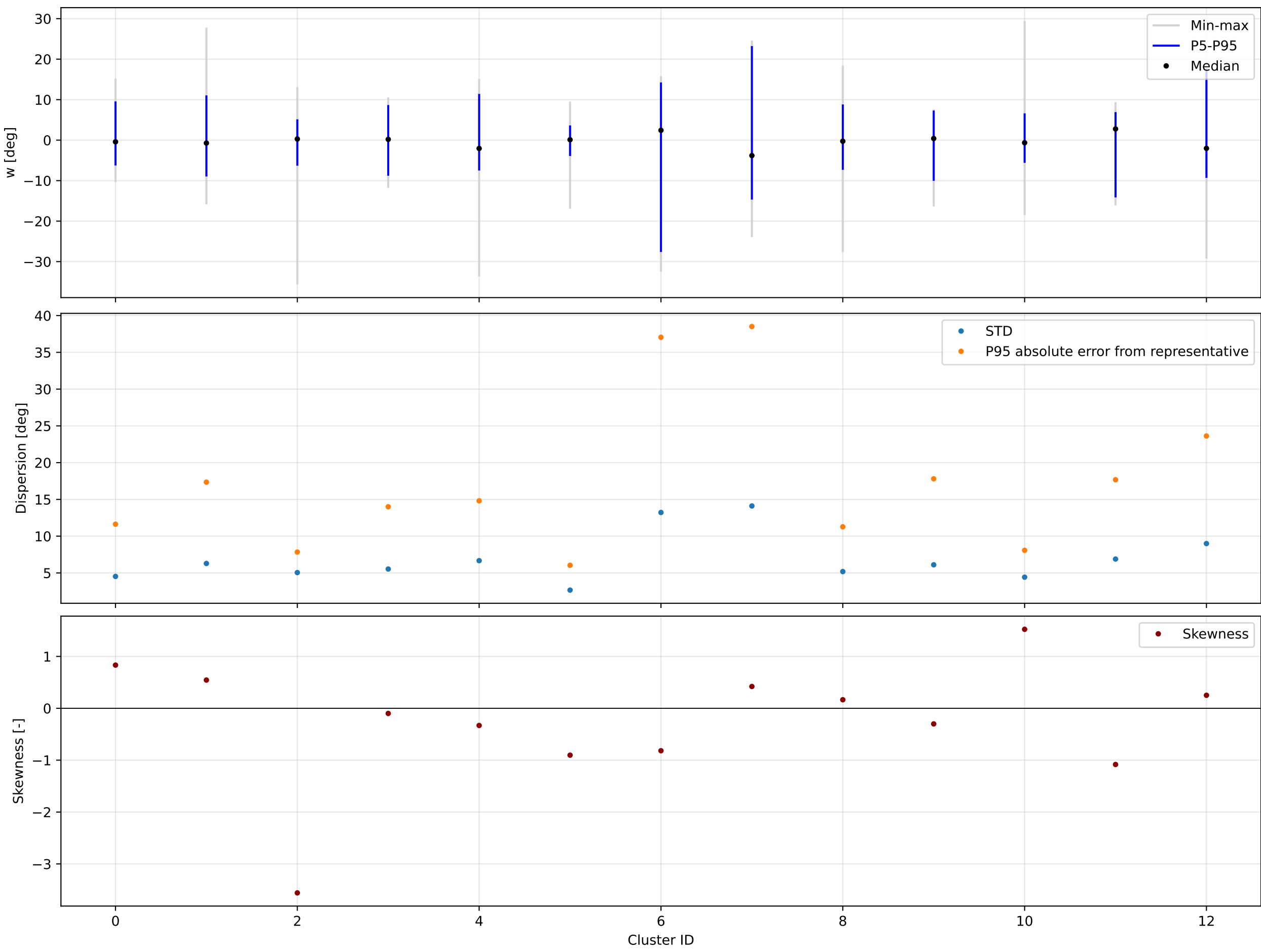
K=13 | backward | w | valid=194124/194124 | offsets from each cluster circular mean
